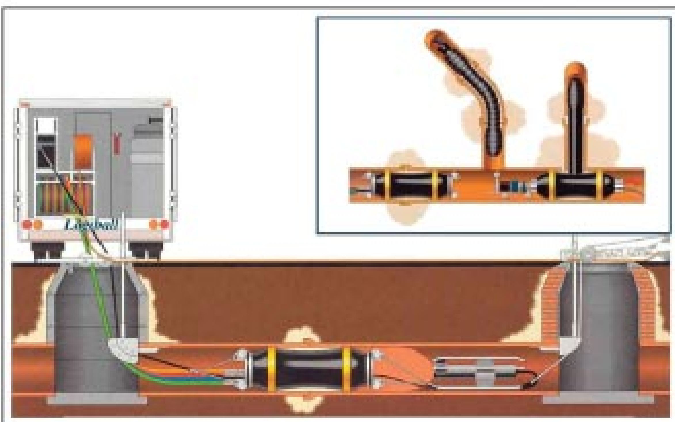
Test and Seal Packers by Logiball Inc.
