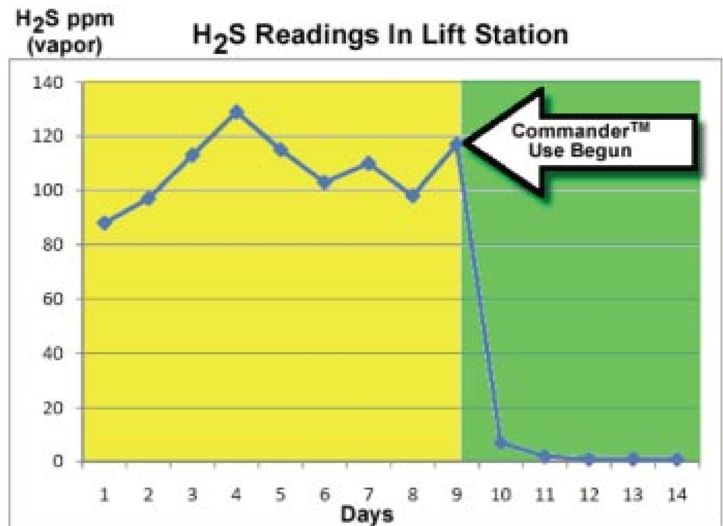
Typical Treatment Response Curve
