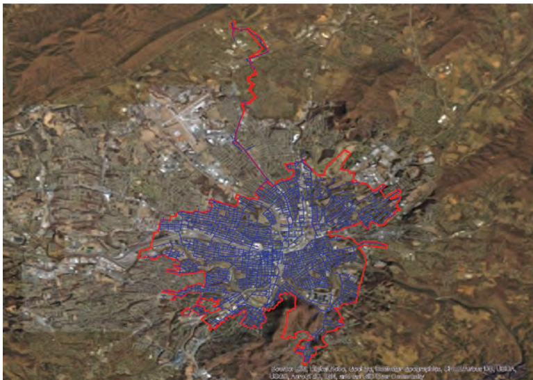
Above: A GIS map of a water utility distribution system. Right: The same distribution system overlaid with likely leak locations as detected by a satellite-mounted radar system. Locations are color-coded according to leak probability.
